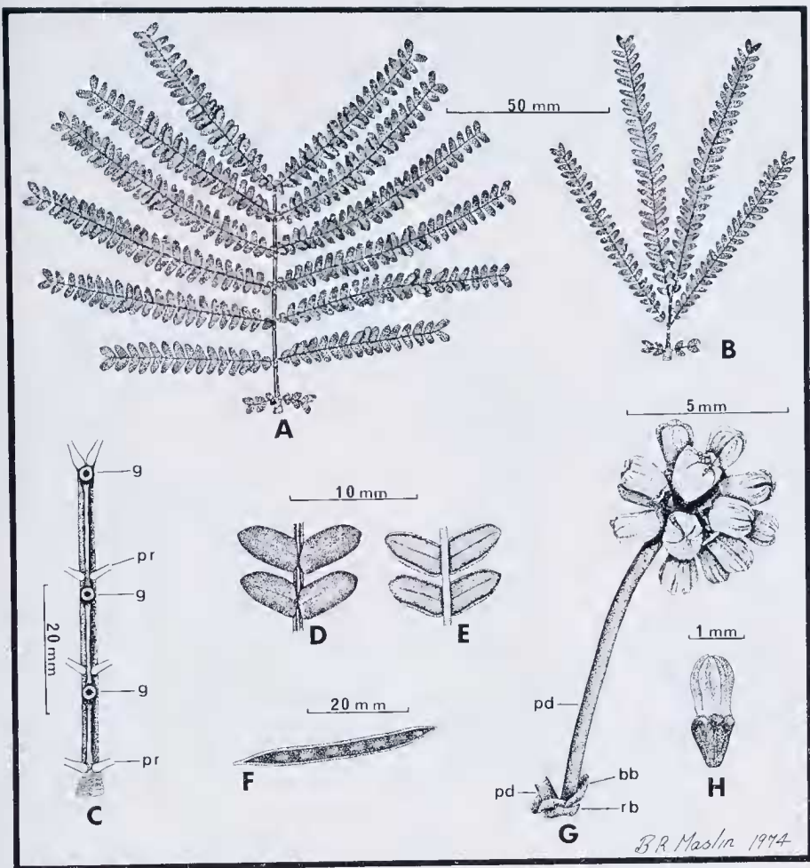
Figure 18— Acacia pentadenia . A and B—Leaves. C—Leaf axis (upper surface) showing glands (g) and base of pinnule rachides (pr). D—Pinnules (upper surface). E—Pinnules (lower surface). F—Legume. G—Inflorescence showing basal bract (bb) subtending peduncle (pd), also solitary bract (rb) subtending the condensed raceme axis. H—Flower. A-E from B. R. Maslin 2896; F from J. W. Green 1135; G-H from A. M. Ashby 2417.
